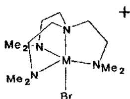
Fig. 7. The trigonal bipyramidal coordination in the species \text{LBr}^+ .
